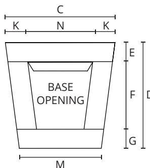
BASE VIEW
