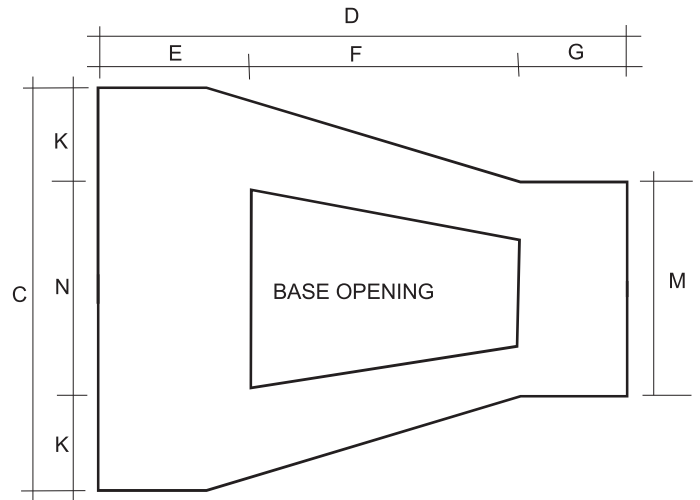
BASE VIEW
